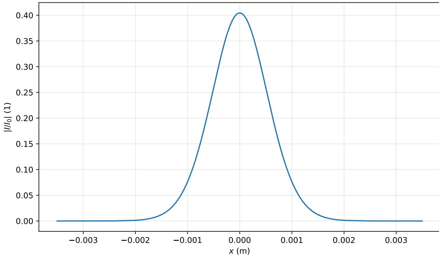
Intensity profile I(x, y = 0, z = 3.105m)/I_0 , P_{in}=0.3P_{cr} , artificial time
